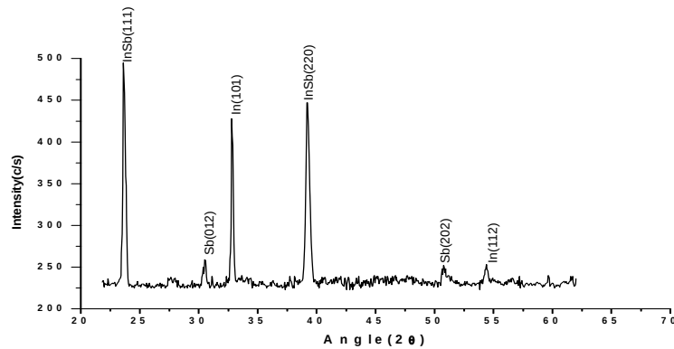
Fig.1(c): X-ray diffraction pattern of as deposited films at 423K.
