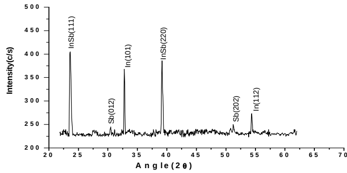
Fig.1(a): X-ray diffraction pattern of as deposited films at 323K.
