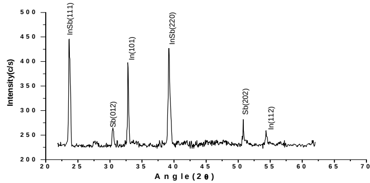
Fig.1(b): X-ray diffraction pattern of as deposited films at 373K.
